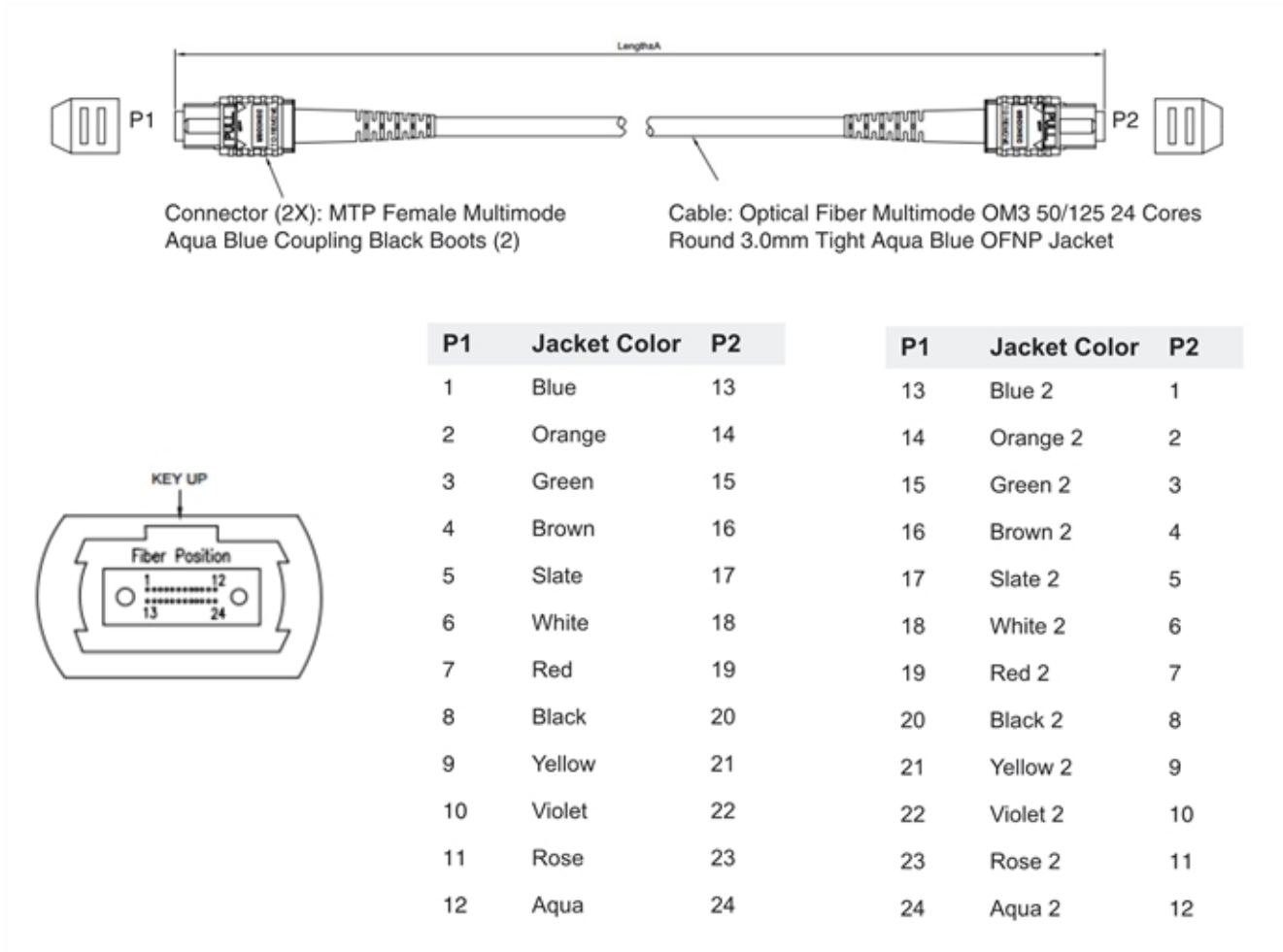
Figure 19 MPO/MTP 24 Position Fiber Cable
