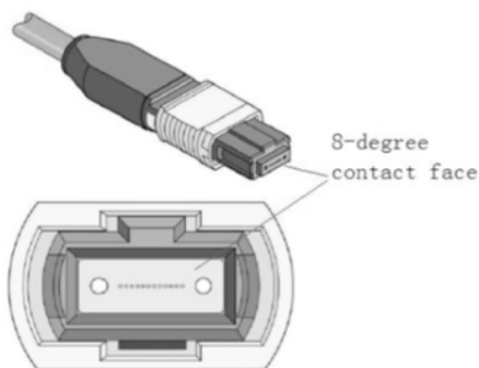
Figure 18 MTP/APC Cable
