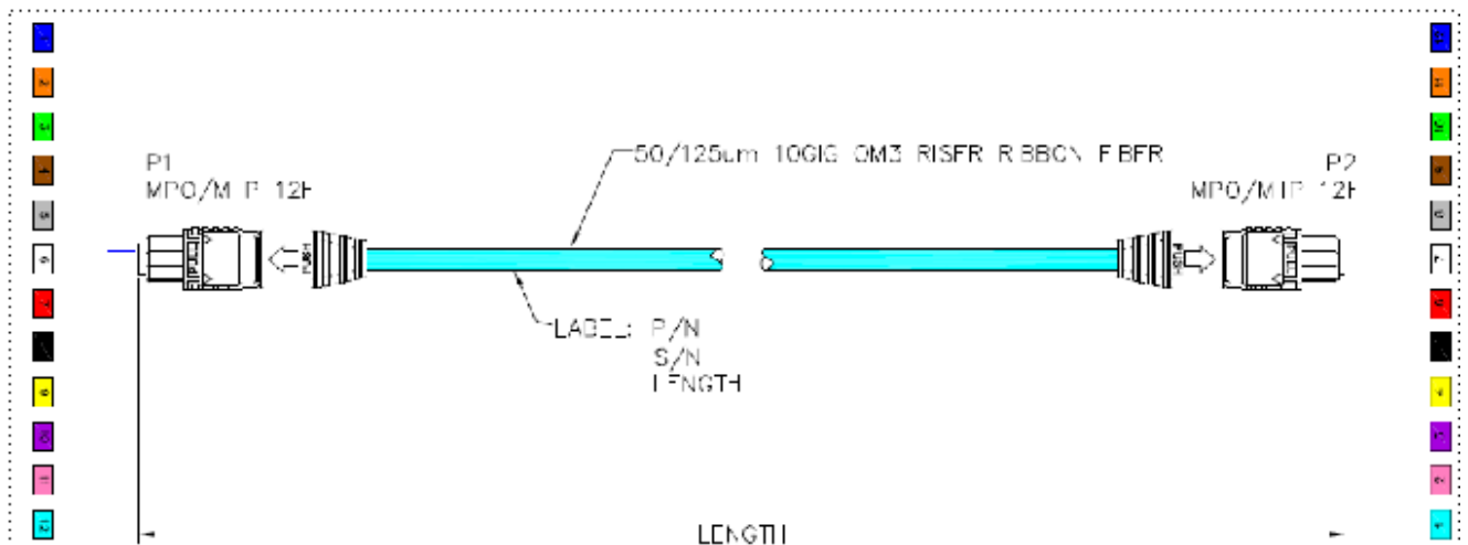
Figure 17 MPO/MTP 12 Position Fiber Cable
